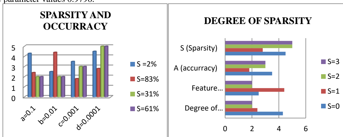
Figure 4.2. SPLR on KDD'20 Feature Selection and Degree of Sparsity
