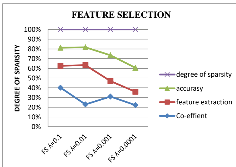
Figure 4.3. KDD '98 Dataset Feature Selection and Degree of Sparsity using SPLR
