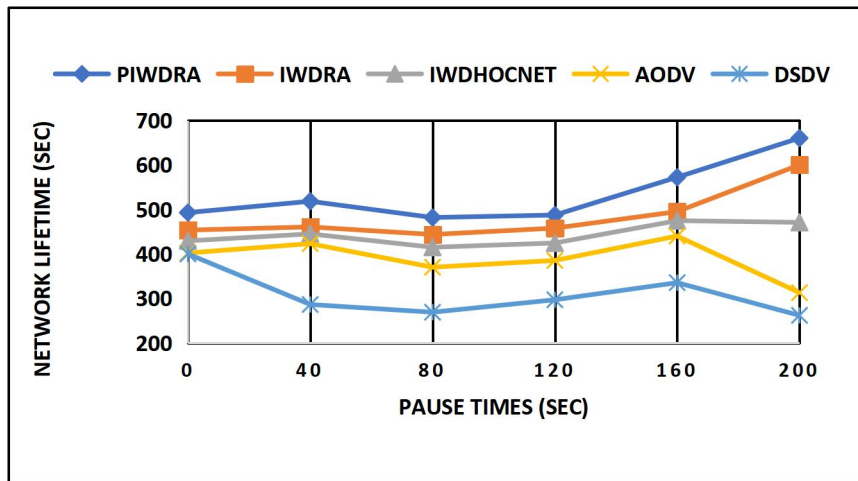
Figure 6. Network Lifetime Under Various Pause Times
