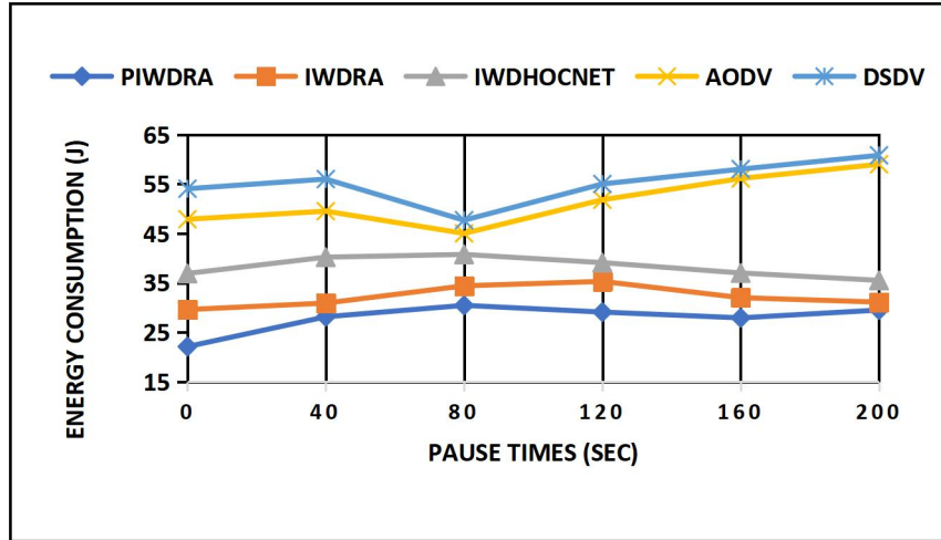
Figure 5. Energy Consumption Under Various Pause Times
