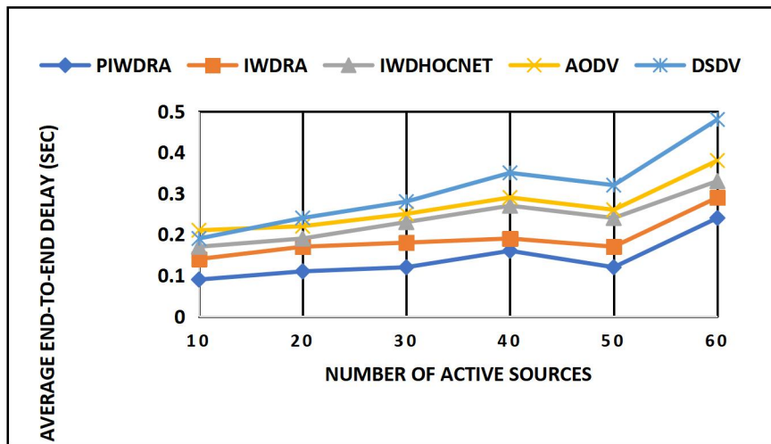
Figure 8. Average End-to-End Delay Under Various Number of Active Sources
