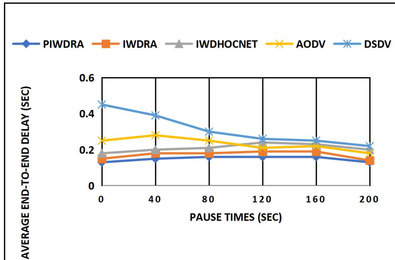
Figure 4. Average End-to-End Delay Under Various Pause Times
