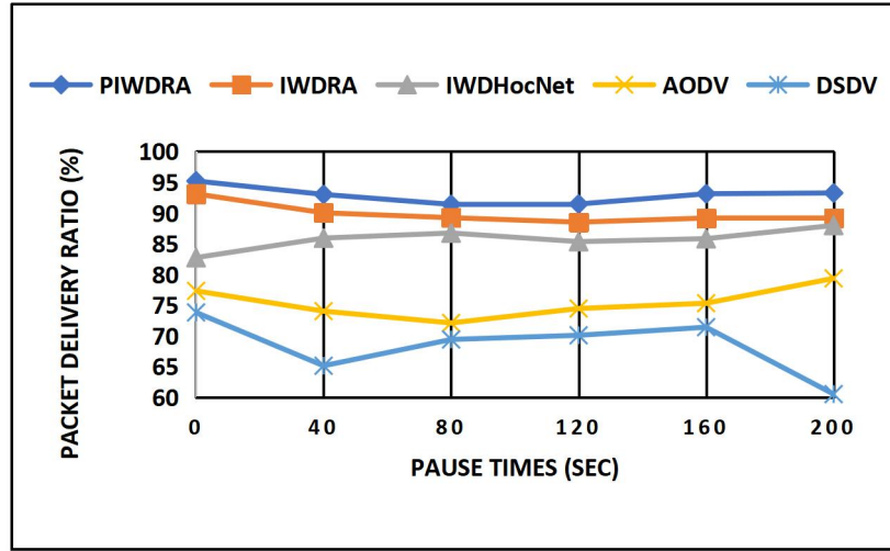
Figure 3. Packet Delivery Ratio Under Various Pause Times
