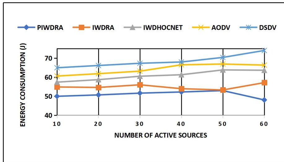
Figure 9. Energy Consumption Under Various Number of Active Sources
