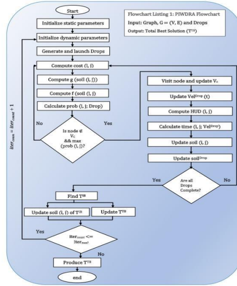
Figure 2. Flowchart of PIWDRA
