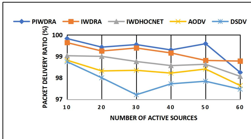
Figure 7. Packet Delivery Ratio Under Various Number of Active Sources
